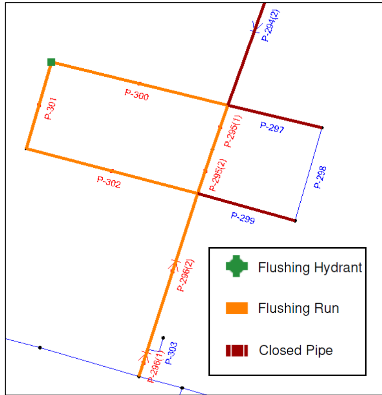
Figure 4-2 Flushing Configuration 2
