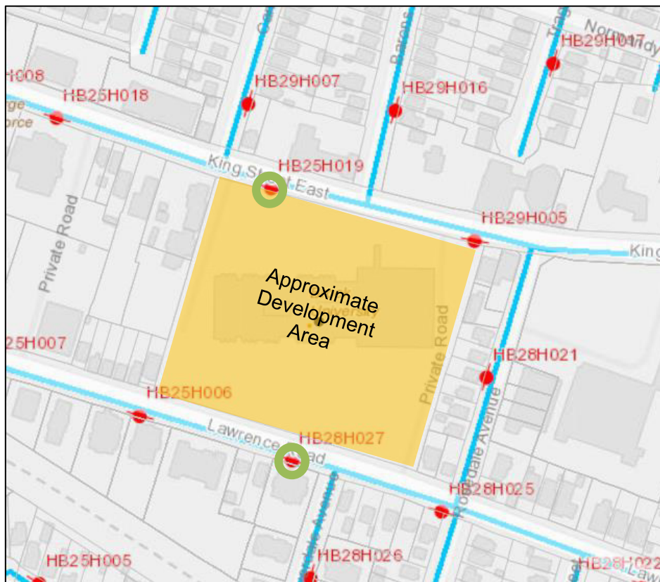
Figure 3-1: Hydrants used for Model Validation
