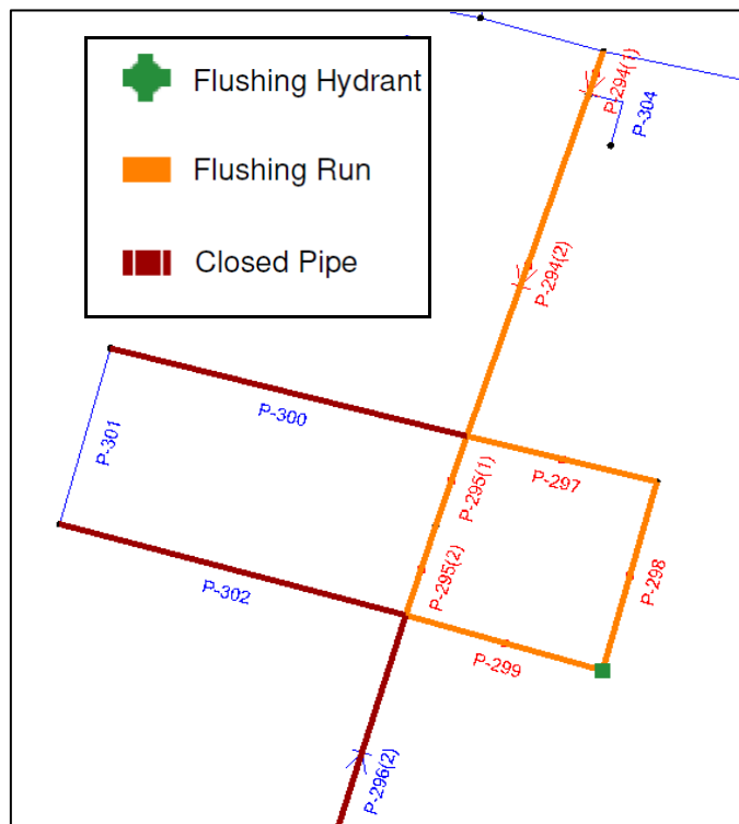
Figure 4-1 Flushing Configuration 1
