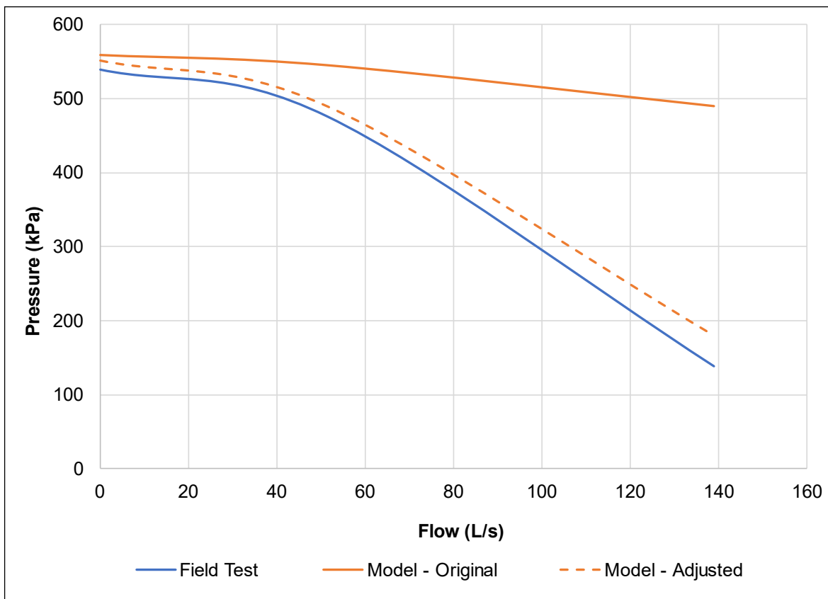
Figure 3-2. Verification Results - Hydrant HA17H038 on John St. North
